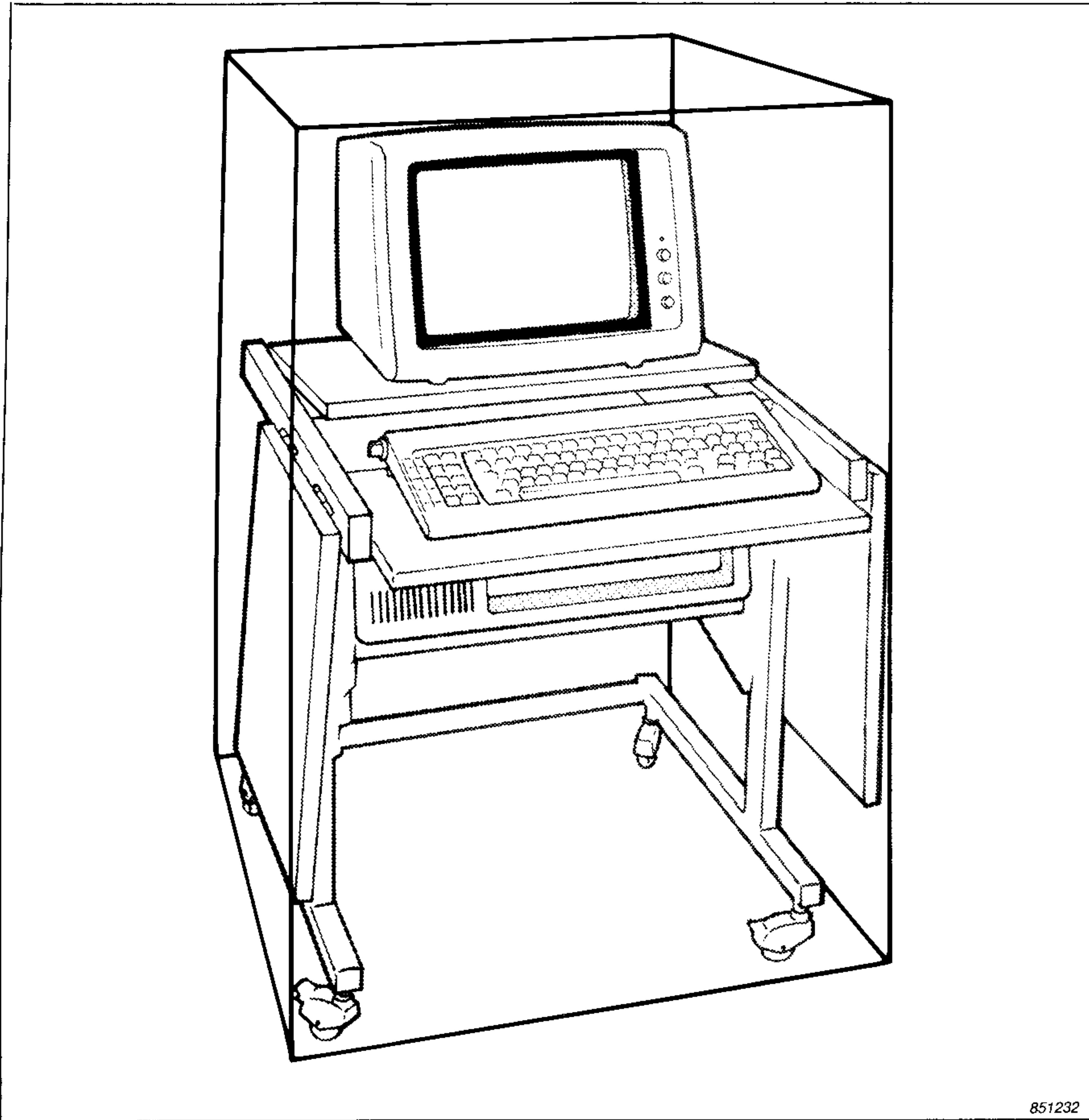
Fig. 5. Measurement surface about a personal computer
