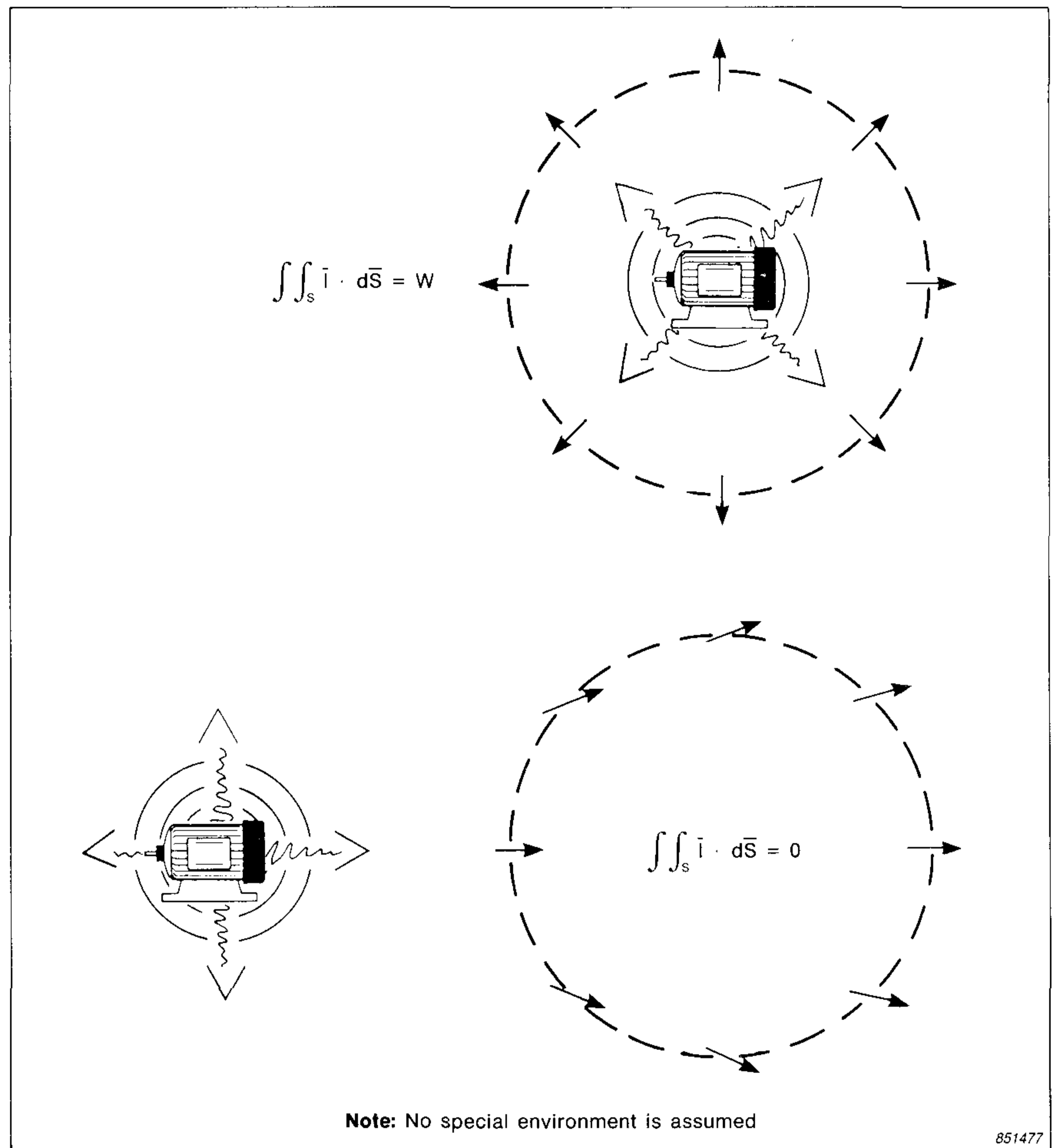
Fig. 3. Principle of measurement of sound power based on sound intensity
