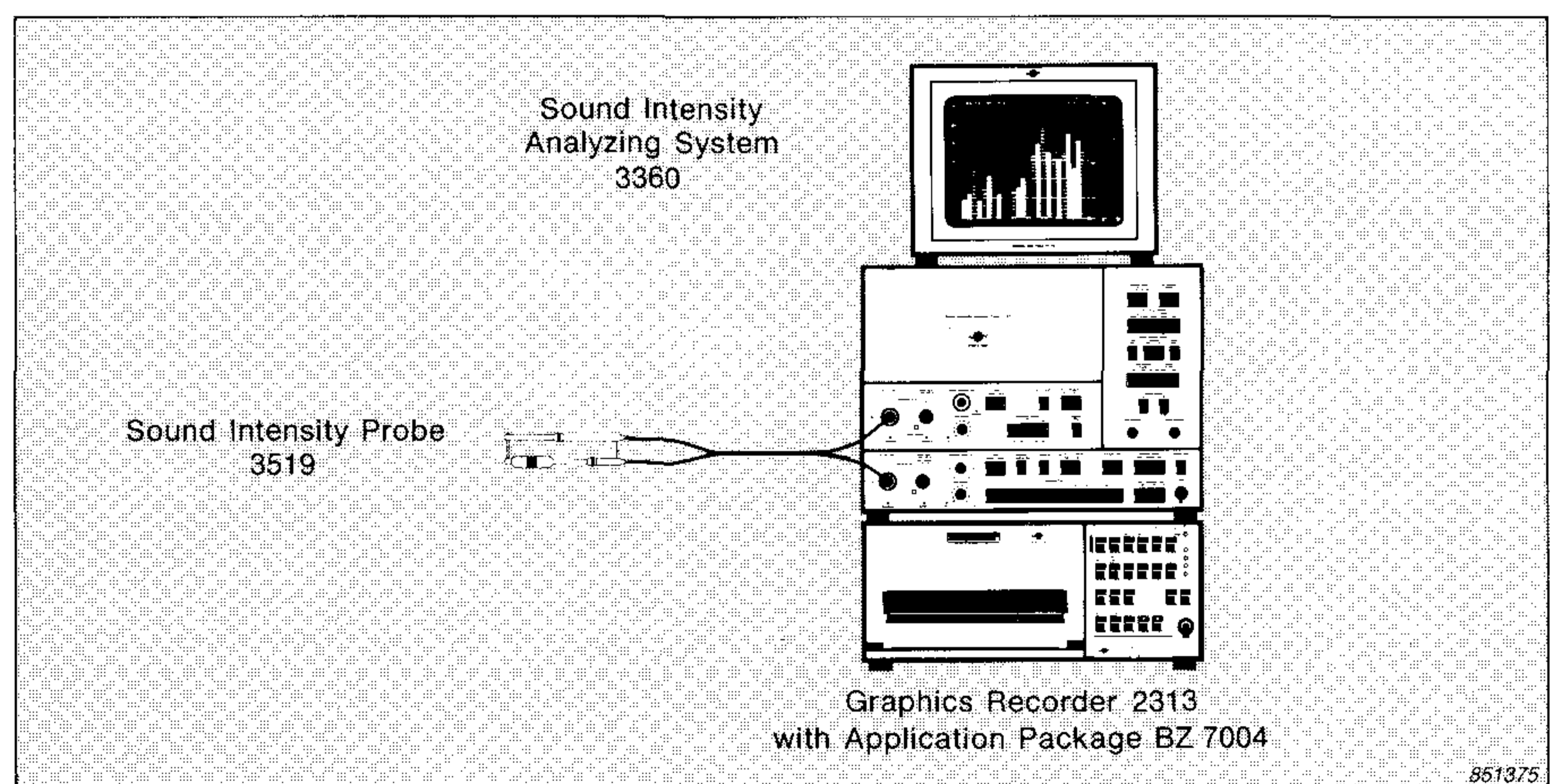
Fig. 4. A system for semi-automatic measurement of sound power based on sound intensity
