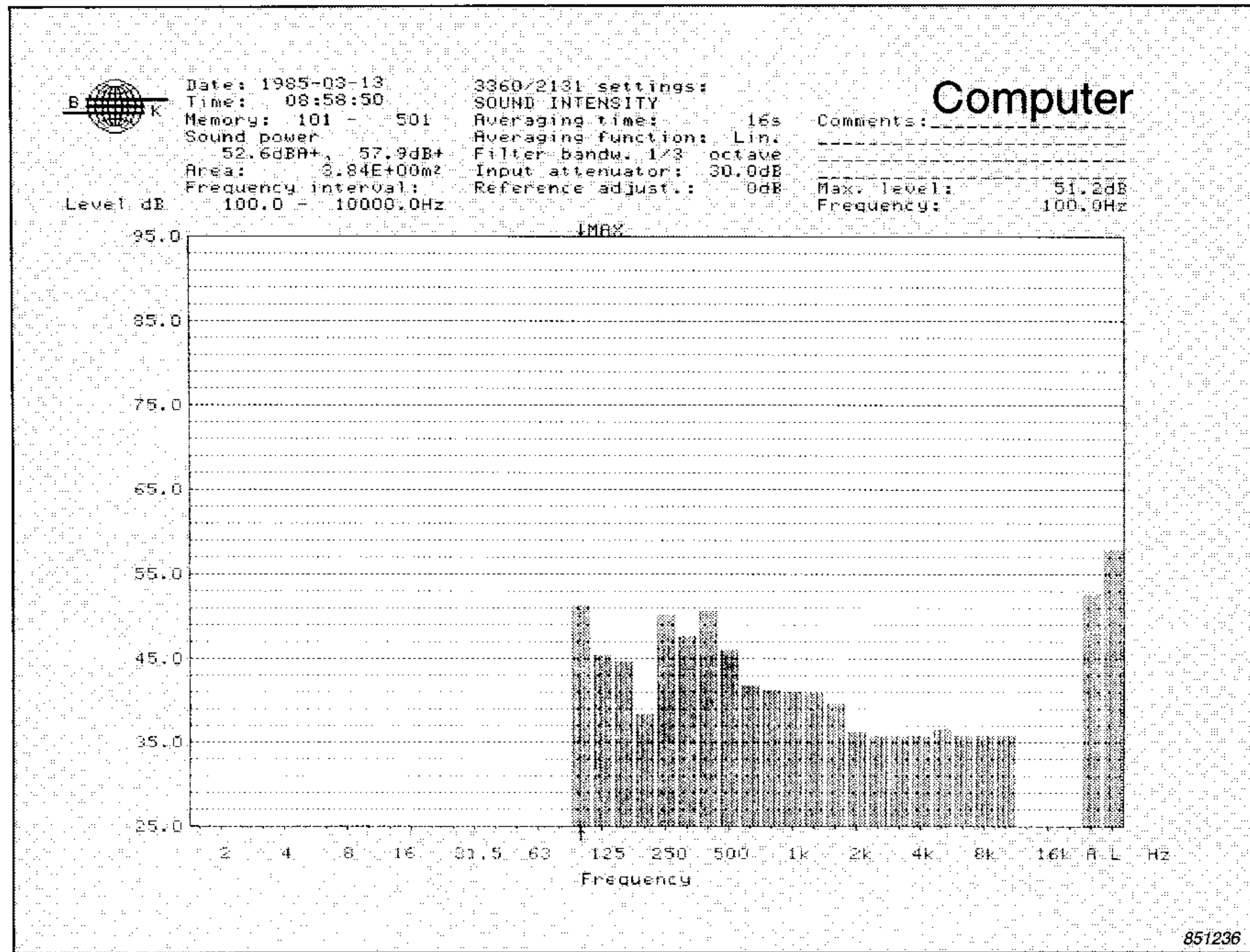
Fig. 7. 1/3 octave plot of the sound power of the personal computer, obtained from the 2313
