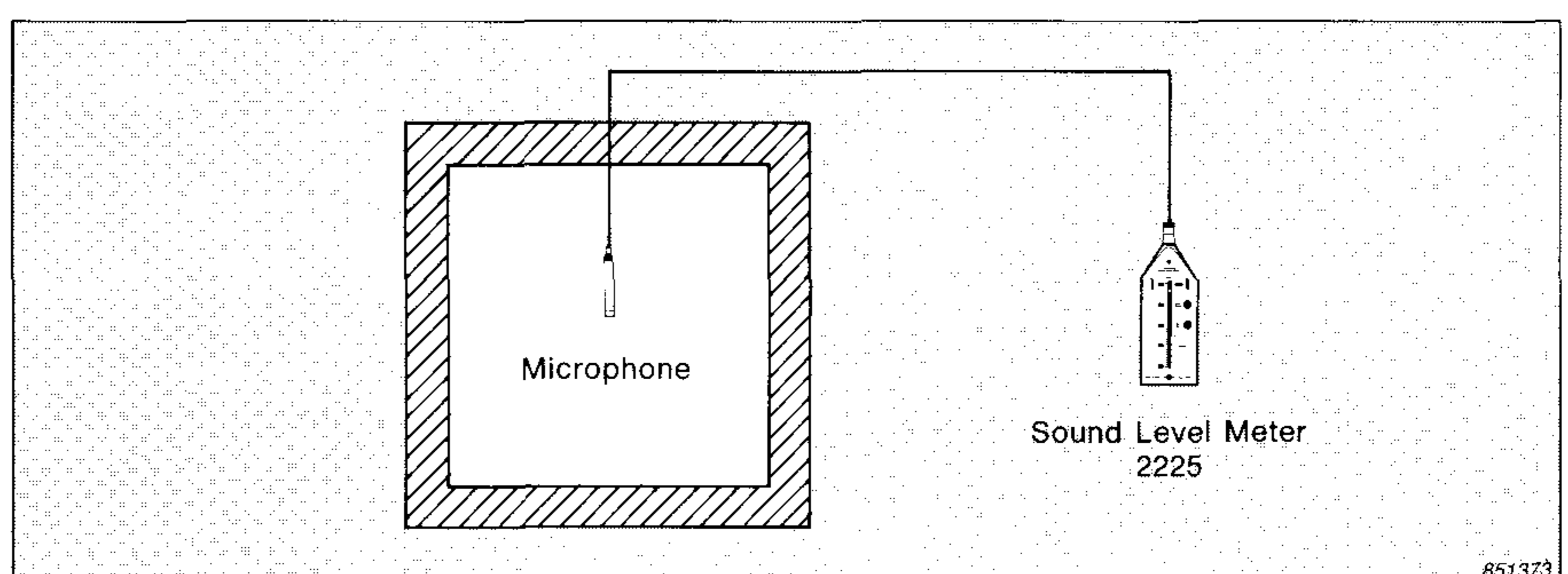
Fig. 1. Use of a test chamber and a sound level meter for production testing
