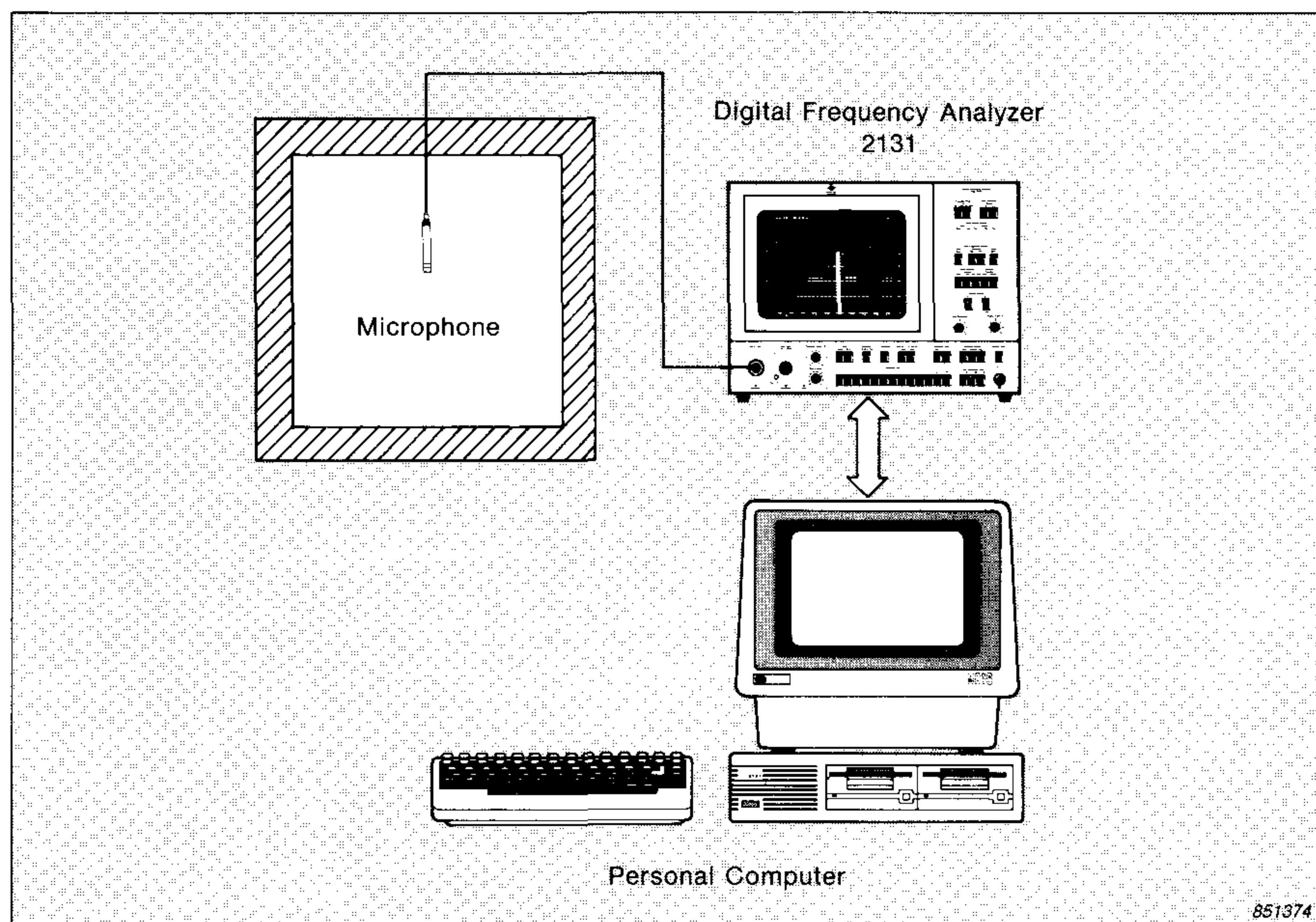
Fig. 2. Production testing system using a real-time analyzer
