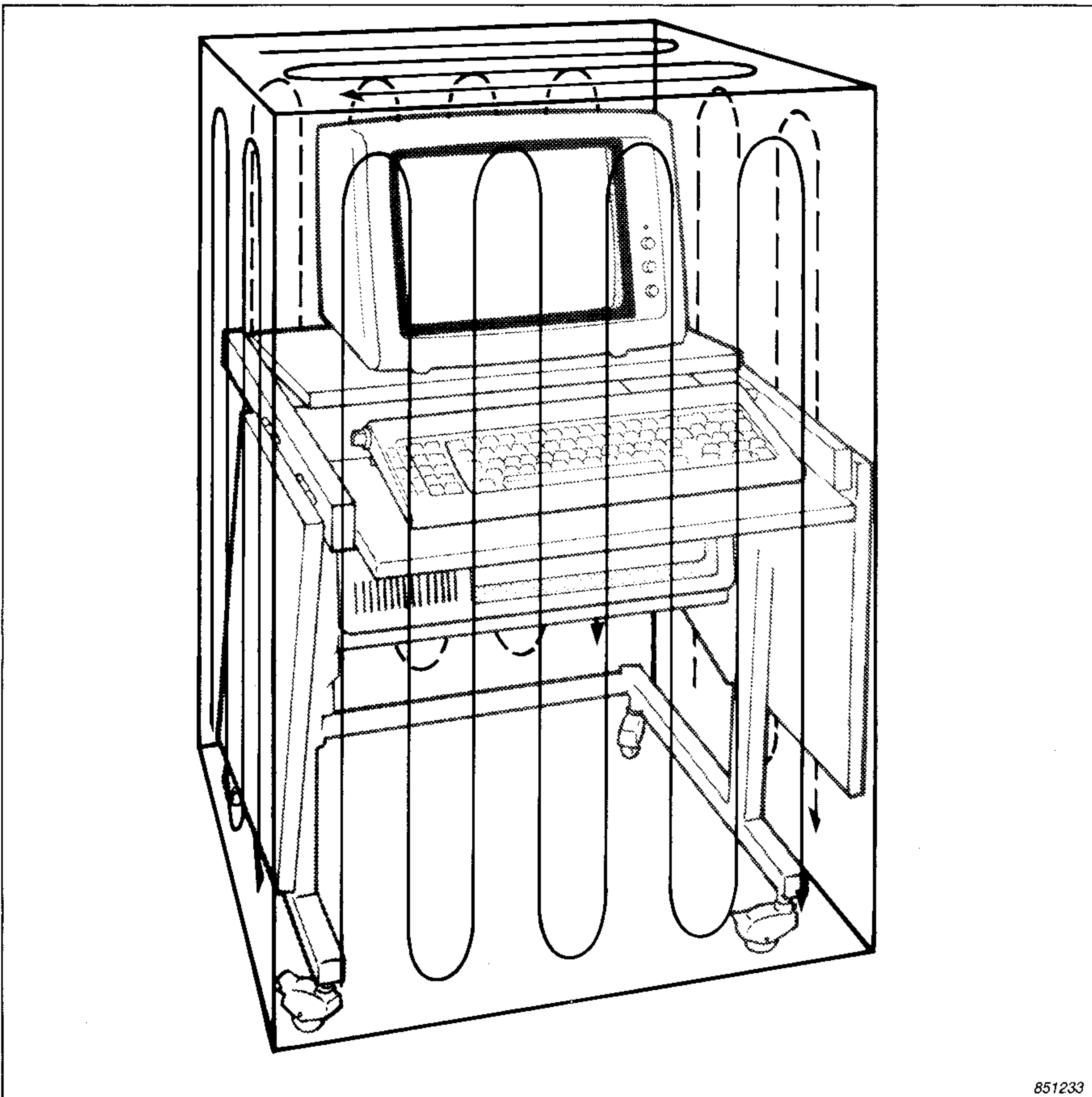
Fig. 6. Measurement of sound power on a personal computer showing the intensity probe's path over the measurement surface
